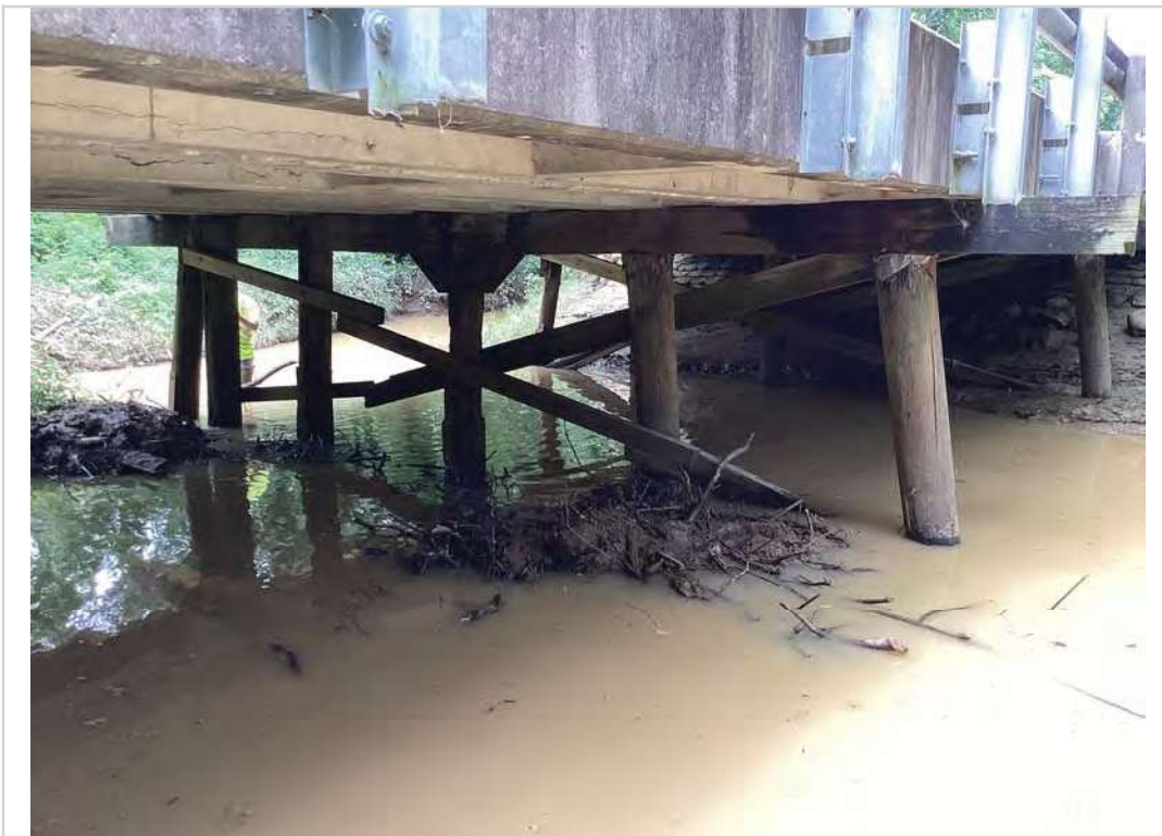
Bent 2 rear
